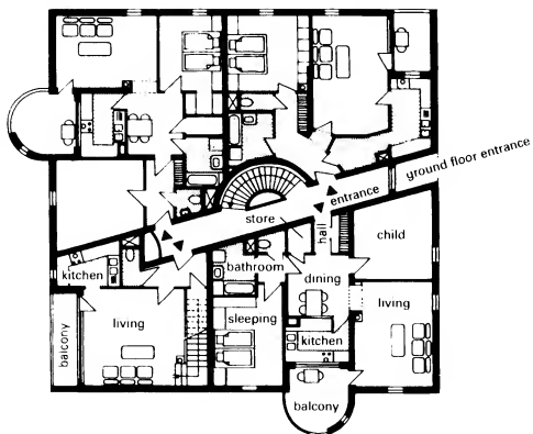
10 Four dwellings per floor
